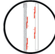
Figure 2 Z-Bar Interlocking Hanging System
